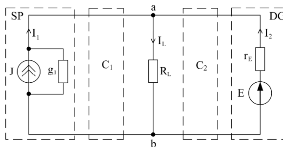
Fig. 1. Simplified equivalent circuit of an autonomous power system.
