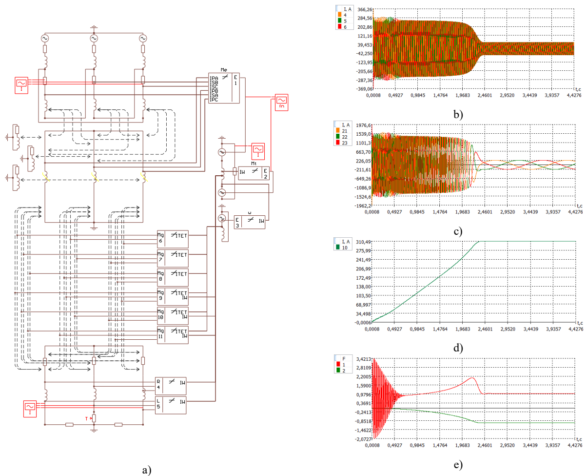
Fig.3. Simulation start-up of the induction motor 310 KW 6.3 kV to the fan load: a) equivalent scheme; b) currents of the stator; c) currents of the rotor; d) the rotor speed; e) electrical and mechanical torques on the shaft of the rotor
