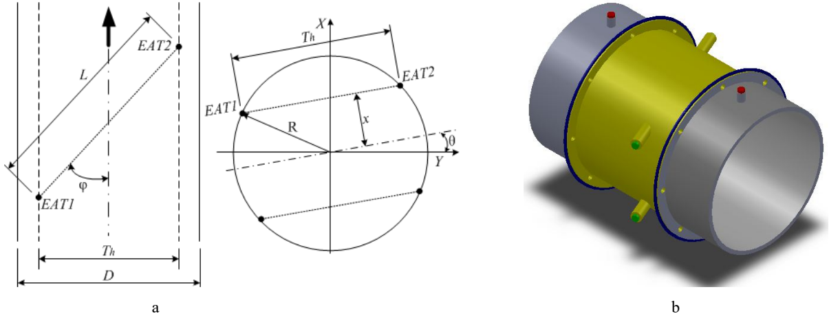
Fig. 1. Simplified design diagram of a double-path chordal USM (a) and three dimensional model of USM and pipe (b) build in CAD software: L – length of the acoustic path; T_h – width of the plane where the acoustic path is located; \varphi – angle of the acoustic path relative to the axis flow; \theta – angle of the acoustic path relative to the horizontal position
