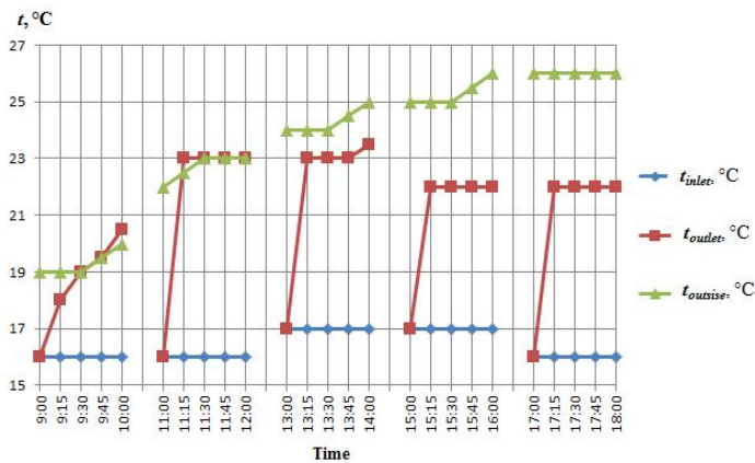
Fig. 3 Changing the heat carrier temperature in the inlet pipe of the solar collector t_{\text{inlet}} , ^\circ\text{C} , in the outlet pipe of the solar collector t_{\text{outlet}} , ^\circ\text{C} and the temperature outside t_{\text{outside}} , ^\circ\text{C} in the southern orientation by strait mode
