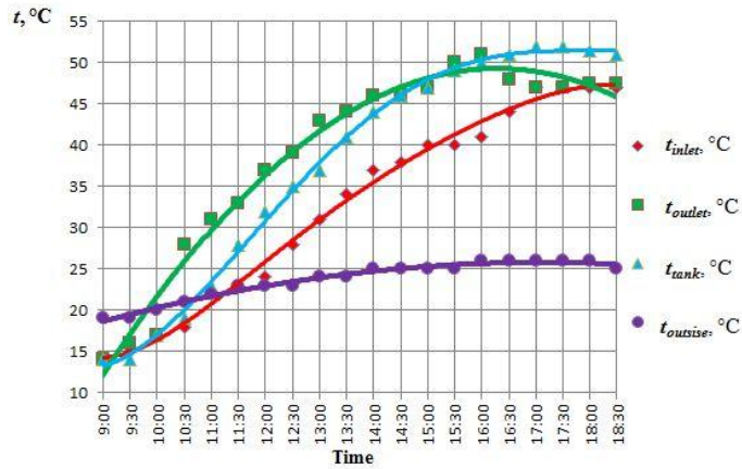
Fig. 2. Changing the heat carrier temperature in the a tank-battery t_{\text{tank}} , ^\circ\text{C} , in the inlet pipe of the solar collector t_{\text{inlet}} , ^\circ\text{C} , in the outlet pipe of the solar collector t_{\text{outlet}} , ^\circ\text{C} and the temperature outside t_{\text{outside}} , ^\circ\text{C} in the southern orientation by gravity mode
