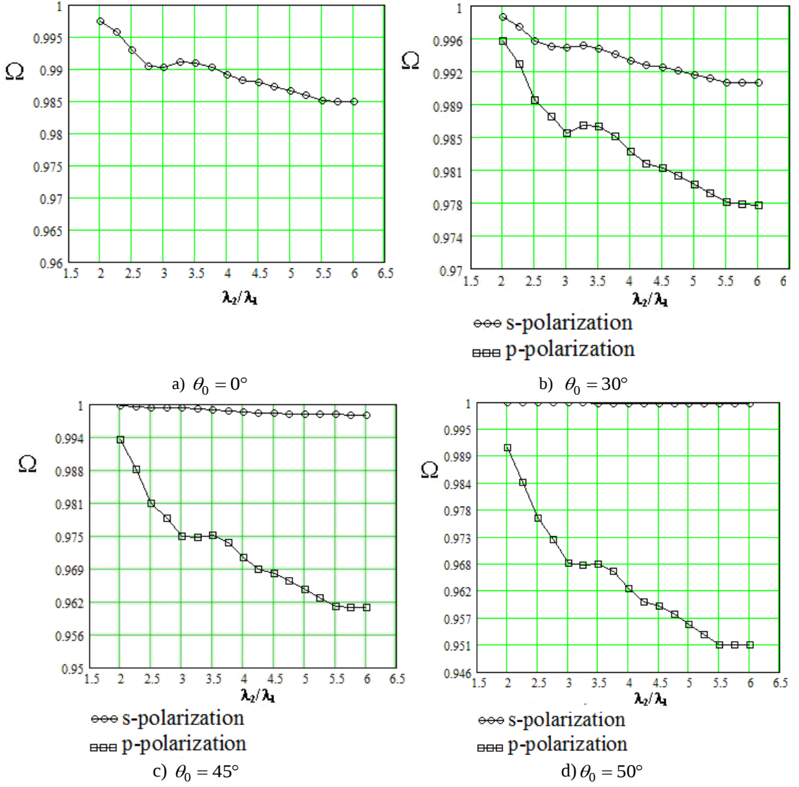
Fig. 1. The dynamics of the change of functional \Omega(\lambda_1, \lambda_2) for four-layer homogeneous structure in cases \theta_0 = 0^\circ , \theta_0 = 30^\circ , \theta_0 = 45^\circ , \theta_0 = 50^\circ
