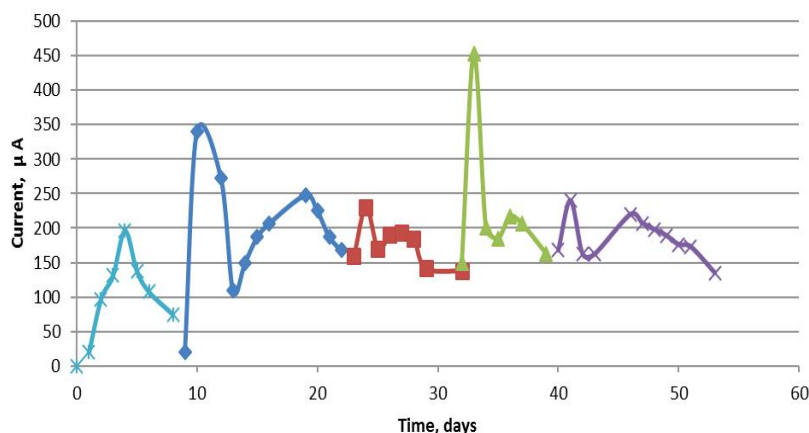
Fig. 1. Current vs. time during the biofilm formation process of electrochemically active microorganisms: —●— start of biofilm formation process; —■— partial replacement of cultural medium 1; —▲— complete replacement of cultural medium; —×— partial replacement of cultural medium 2
