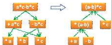
Fig. 2. Expression factorization.
