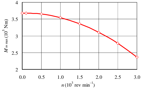
Fig. 12. Dependence of the maximum transferable torque M_{m\text{max}} on the revolutions n ( \Delta r_{AB} = 0.2 \text{ mm} ).
