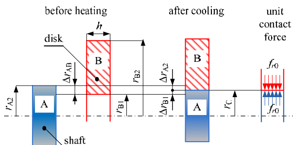
Fig. 1. Preparation of a shrink fit.
