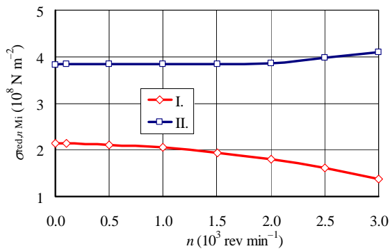
Fig. 11. Dependence of the von Mises stress \sigma_{\text{red},n\text{Mi}} as a function of revolutions n : I – shaft, II – disk ( \Delta r_{AB} = 0.2 \text{ mm} ).
