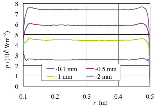
Fig. 18. Distribution of volumetric Joule losses p_J in the disk along its surface in different depths at the beginning of the heating process ( T_0 = 30^\circ \text{C} , I = 2.5 \text{ kA} ).
