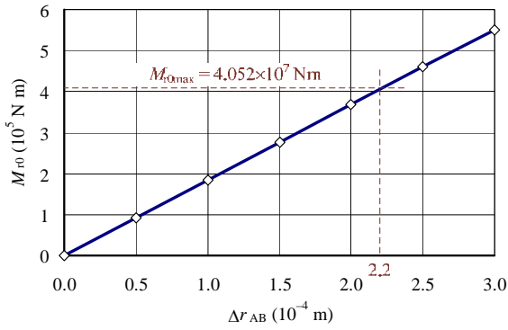
Fig. 10. Transferable torque M_{T0} of the shrink fit (at rest) as a function of \Delta r_{AB} .
