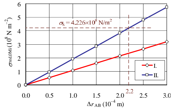
Fig. 9. Von Mises stress \sigma_{red,0Mi} in the system at rest as a function of \Delta r_{AB} : I – shaft (here \sigma_{red,0Mi} = f_{r0} ), II – disk.
