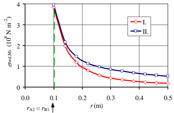
Fig. 13. Dependence of the von Mises stress \sigma_{\text{red,Mi}} in the disk on the radius I – at rest ( n = 0 ), II – at nominal revolutions n_0 = 3000 \text{ rpm} ( \Delta r_{AB} = 0.2 \text{ mm} ).
