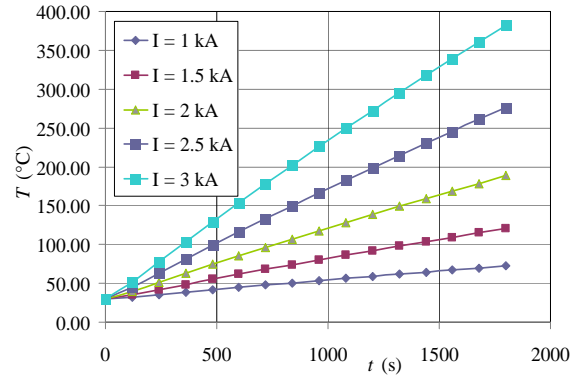
Fig. 21. Time evolution of average temperature T in the disk for various amplitudes I of the field current.
