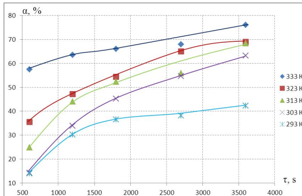
Fig. 1. Conversion level of kainite vs. time at different temperatures
