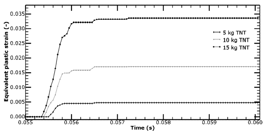
Fig. 10. Time history of maximum equivalent plastic strain
