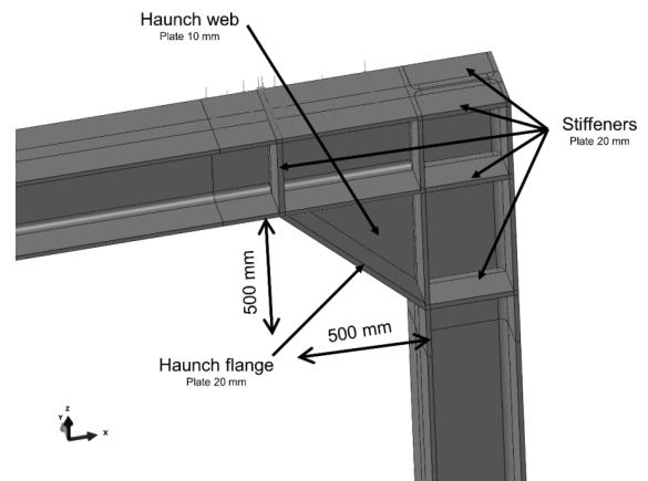
Fig. 2. Detail of frame corner
