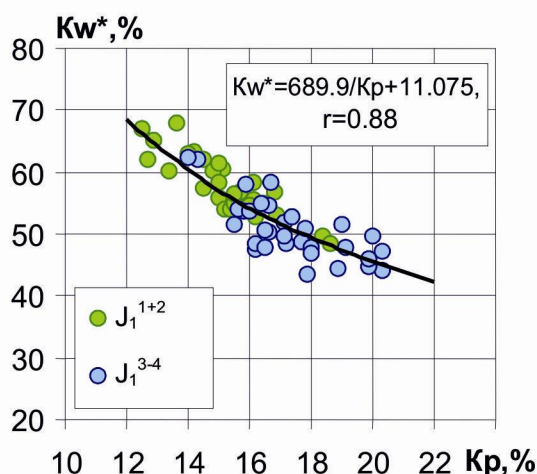
Fig. 2. Standard dependence of critical water saturation value K_w^* from K_p for the layers of the Jurassic horizon [Serjenga, 2007]
