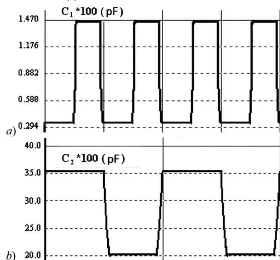
Figure 11. An example of the C_1 (a) and C_2 (b) capacity changes in time due to acceleration
