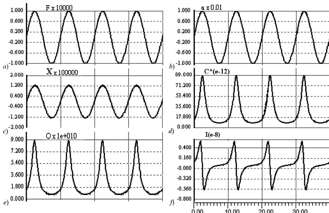
Figure 9. An example of the force magnitude changes (N) in time (a), of the acceleration changes in time under the applied force (b), of the shift changes (μm) (c), capacity (pF) (d), charge (e) and of the current changes (A) (f) in time due to acceleration
