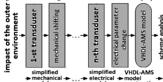
Figure 5. Scheme of synthesis method of VHDL-AMS models for electromechanical MEMS devices
