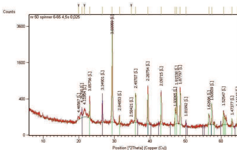
Fig. 11. Diffractogram of hard material.
