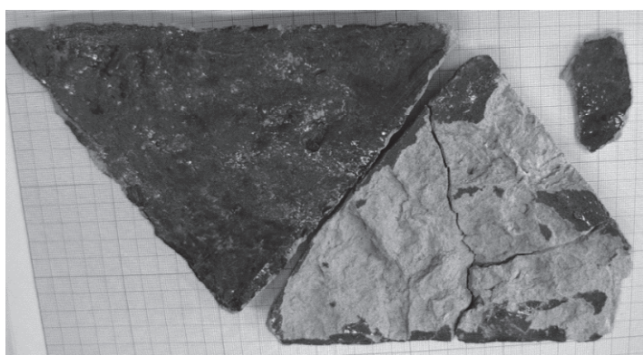
Fig. 4. Building materials obtained from materials synthesized from Cholm chalk. Fragment of a brick or architectural detail (a), glazed tiles (b).
