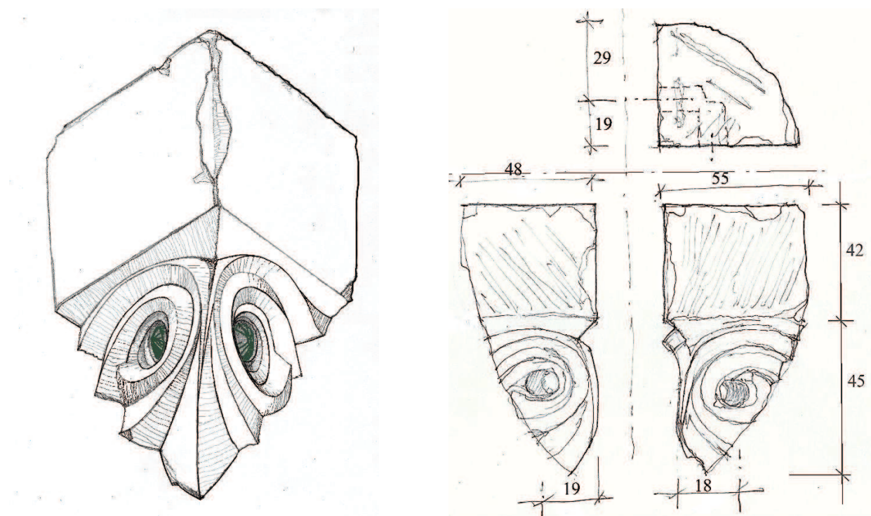
Fig. 1. Fragment of a carved detail of white limestone (fragment of the capital? Excavation Ch/G/W-67/2016) with drilled holes and inserts of green glaukonitite sandstone (prepared by M. Bevz).
