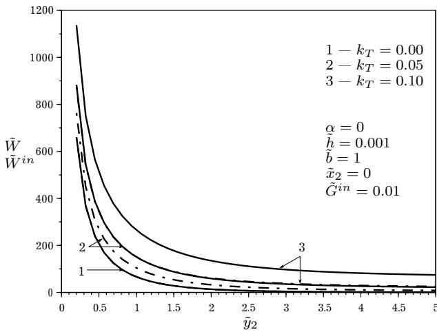
Fig. 2. Effect of coefficient on the energy of deformation \tilde{W}^d of the matrix (solid curve) and the inclusion \tilde{W}_{in}^d (dashed-dotted curve) when the dislocation is distanced from the axis of the soft inclusion.
