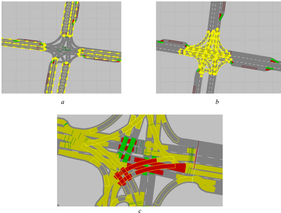
Fig. 7. Creation of an intersection model in the PTV VISSIM software: a – creation of approaches to the intersection; b – creation of sections of roads within the intersection; c – creation of departure priorities.
