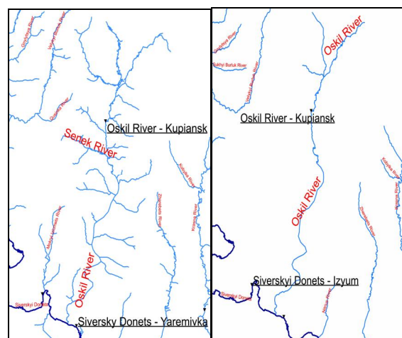
Figs. 3, 4. The influence of scale on the detail of the hydrographic network (for example, the Oskil River)
